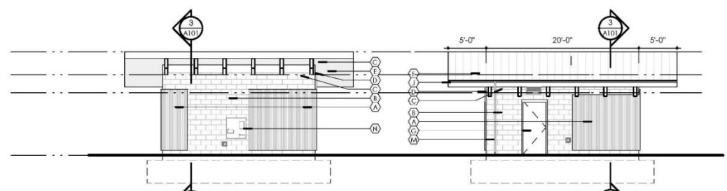
8 NORTH ELEVATION A101 1/8" = 1'-0"
